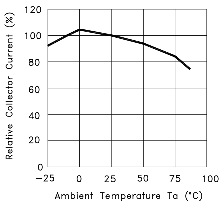
Fig.4 Collector Current I C vs. Ambient Temperature
