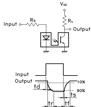
Test Circuit for Response Time
